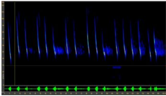
Whiskered or Brandt's Bat call (left), against known Alcaethoe Bat calls (right)
